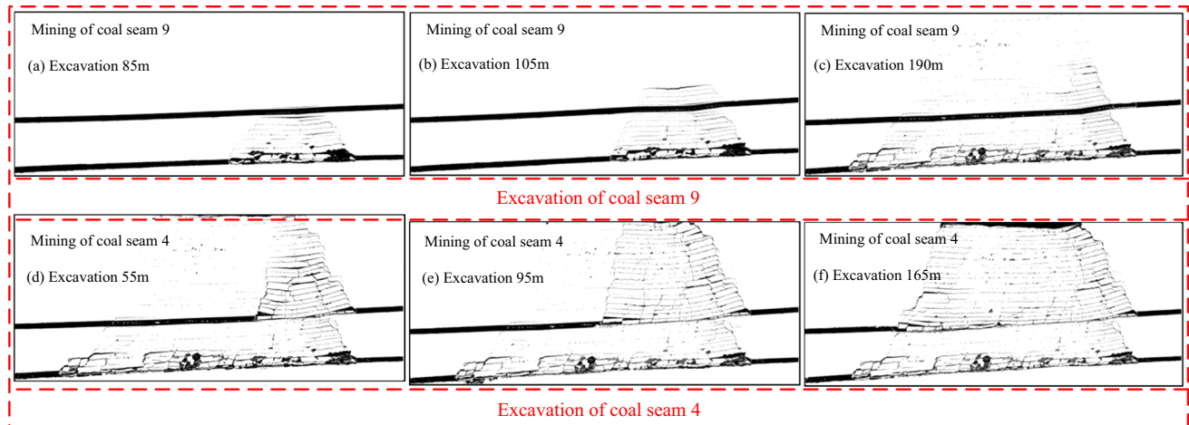
Fig. 5 Overburden Fracture Characteristics of coal seams 4 and 9 in Downward Mining
